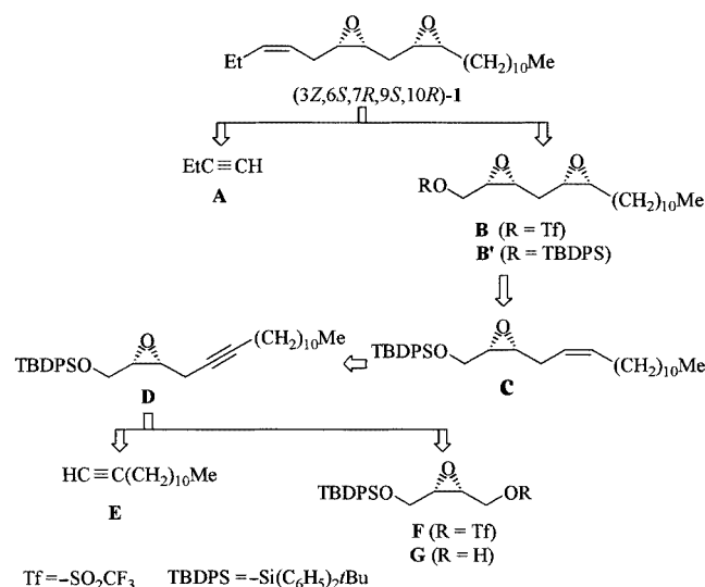
Scheme 2. Retrosynthetic analysis of (3Z,6S,7R,9S,10R)-leucomalure ( 1 )
