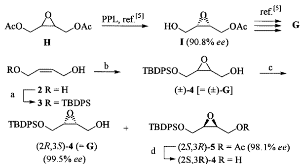
Scheme 3. Synthesis of the enantiomers of epoxy building block 4 . Reagents: (a) NaH, TBDPSCl, THF (92%); (b) MCPBA, \text{CH}_2\text{Cl}_2 (94%); (c) Lipase PS-C, \text{CH}_2=\text{CHOAc} , \text{Et}_2\text{O} [(2R,3S)- 4 (49%) and (2S,3R)- 5 (48%)]]; (d) \text{K}_2\text{CO}_3 , MeOH (99%)
