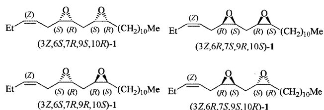
Scheme 1. Structures of the stereoisomers of leucomalure
