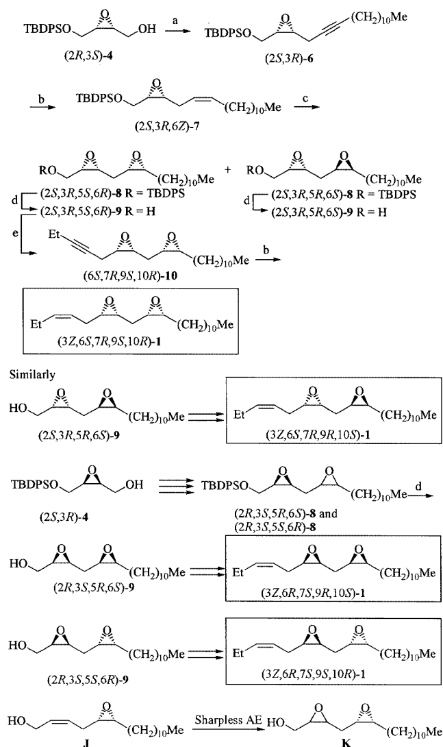
Scheme 4. Synthesis of all the four stereoisomers of leucomalure (1). Reagents: (a) n BuLi, TiF 4 ; then Me(CH 2 ) 10 C≡CLi, THF, HMPA (77%); (b) H 2 , Pd/CaCO 3 -Pb 2+ , cyclohexane [98% for (2S,3R,6Z)-7; 97% for (3Z,6S,7R,9S,10R)-1]; (c) MCPBA, CH 2 Cl 2 ; then MPLC separation [(2S,3R,5S,6R)-8 (23%) and (2S,3R,5R,6S)-8 (58%)]; (d) TBAF, THF (81%); (e) n BuLi, TiF 4 ; then EtC≡CLi, THF, HMPA (48%)
